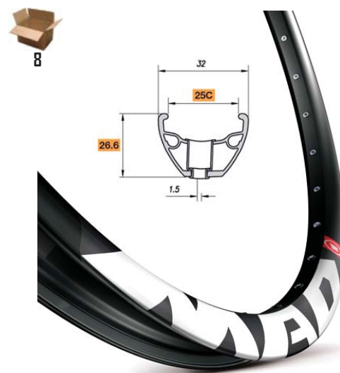
R2136C0015P86M62155932.....28,80 € LLANTA 26" MACH1 MAD DISC (559 x 25C) ALUMINIO, 32H. ERD 534 mm. Negra
