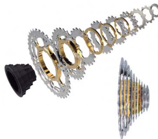
R3987C0032P88MFE9X.....59,70 € PIÑÓN ROSCA 9V. (11-32T.) E-BIKE Chrome
